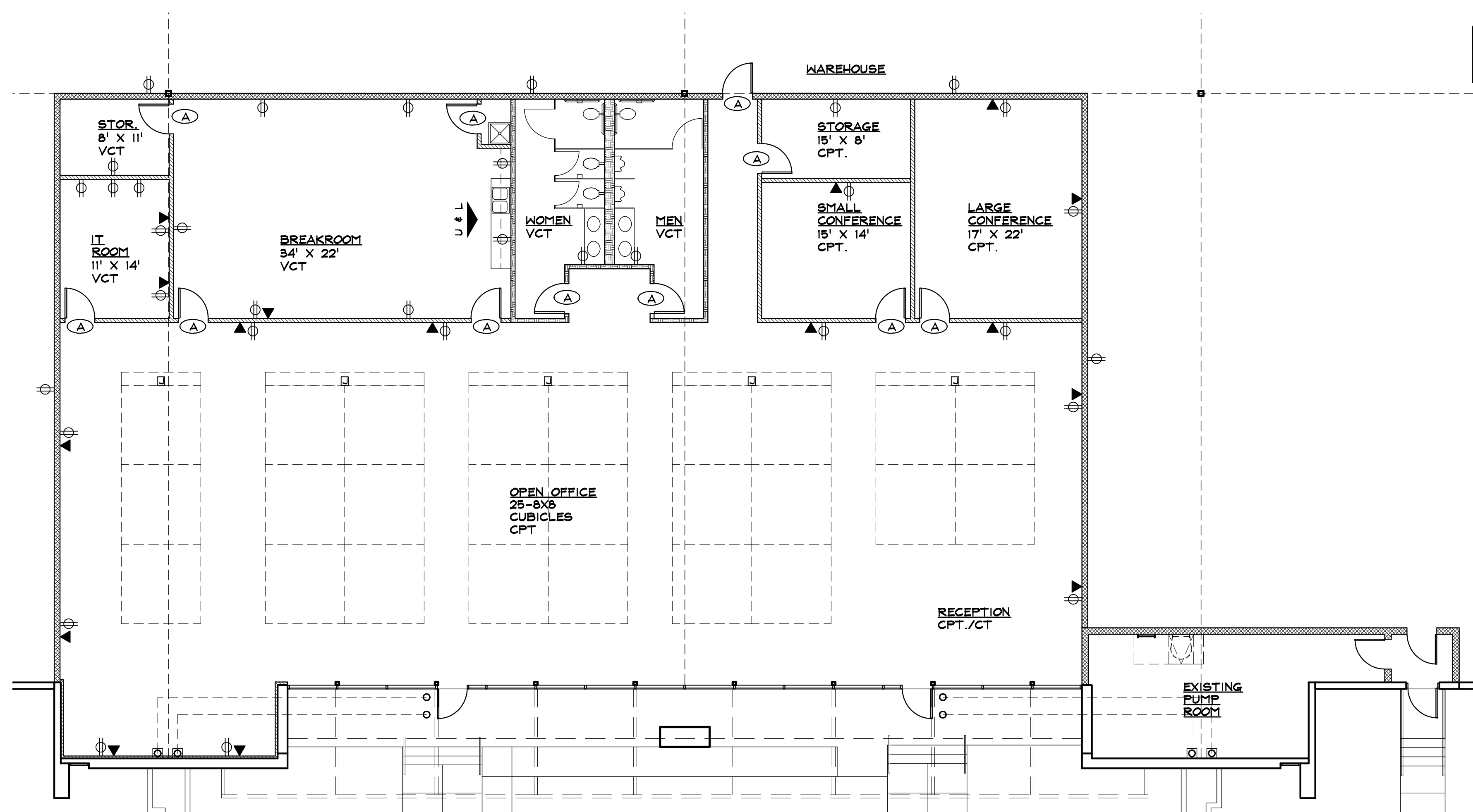
02 OFFICE PLAN Scale: 1/8" = 1'-0" NORTH
