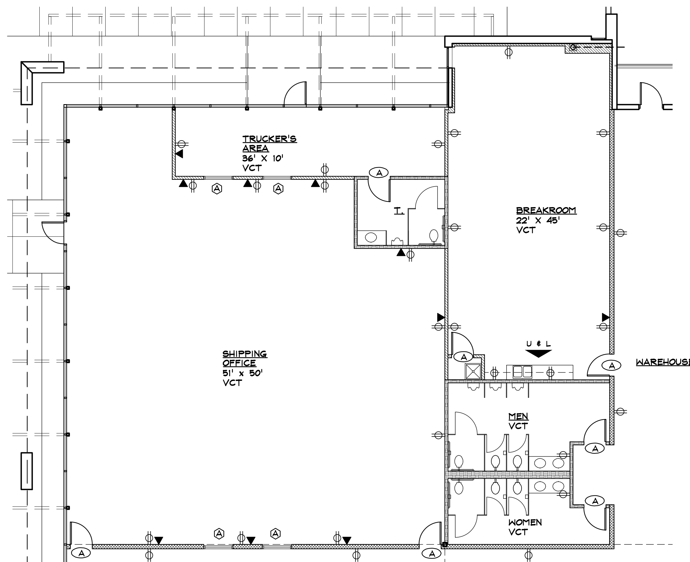
01 WH OFFICE PLAN Scale: 1/8" = 1'-0" NORTH
