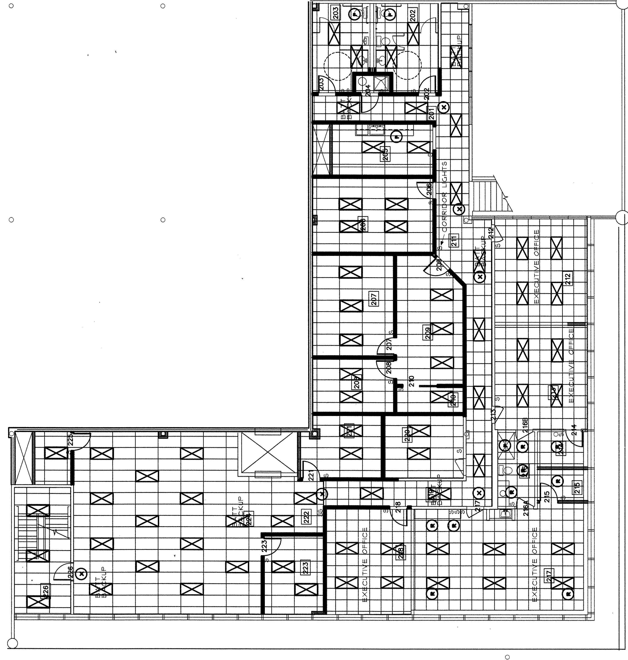
2ND FLOOR REFLECTED CEILING PLAN
