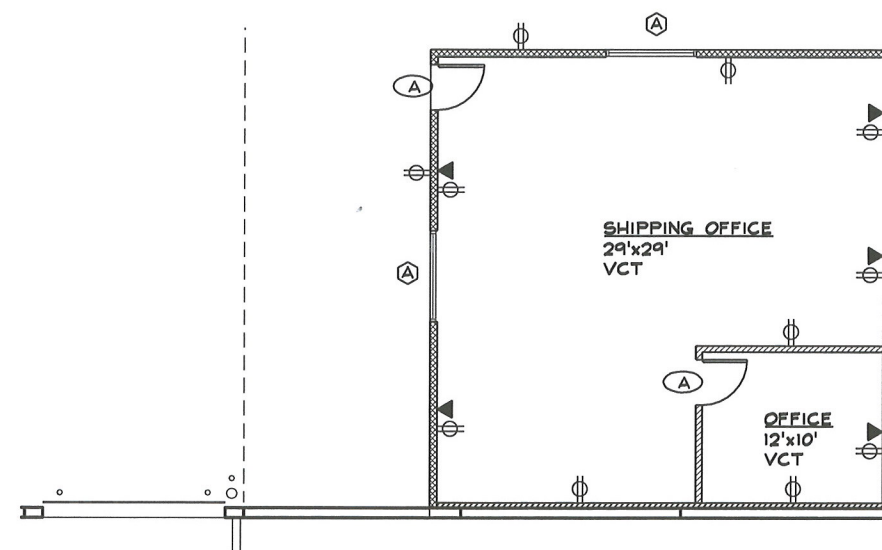
03 SHIPPING OFFICE 1/8" = 1'-0" NORTH
