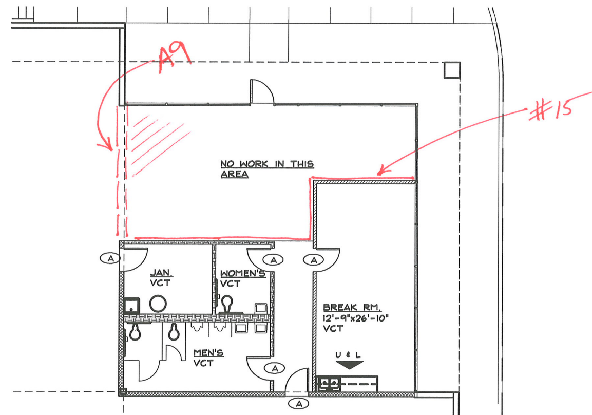
02 SUPPORT OFFICE 1/8" = 1'-0" NORTH
